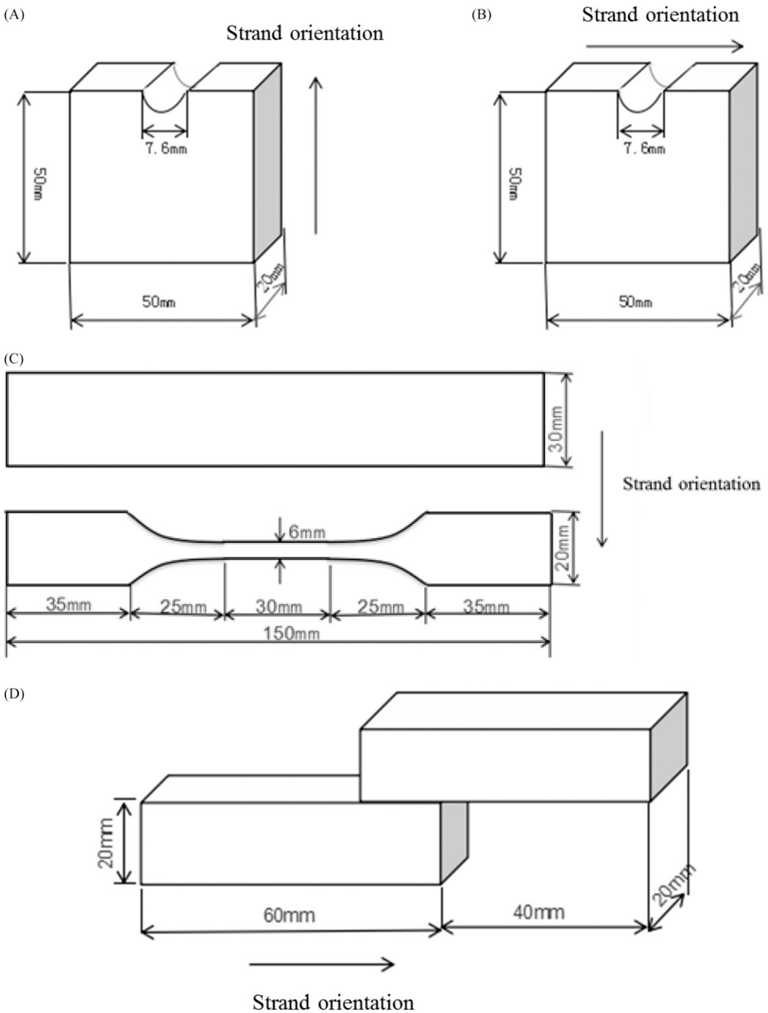
Figure 2. General configurations of half-hole specimens for evaluating bolt-bearing strength of PBSPs parallel (a) and perpendicular (b) to bamboo grain orientation, tensile (c), and shear (d) strength specimens.
