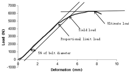
Figure 10. A typical load-deformation curve of single-bolt connections.
