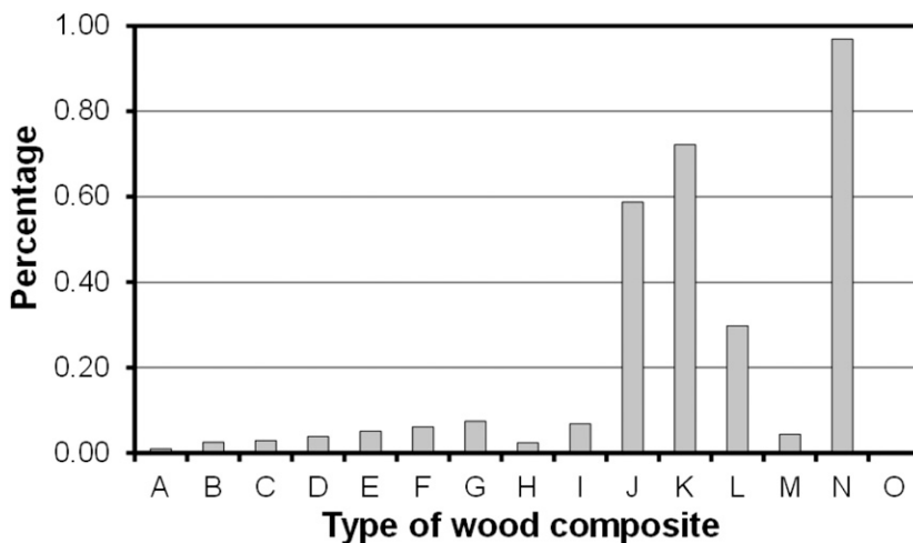
Figure 8. Content percentages of dust particles with a size of 2.5 to 10 \mu\text{m} in the dust created during the milling of wood composites ( C_i = 2,5-10 \mu\text{m} ).
