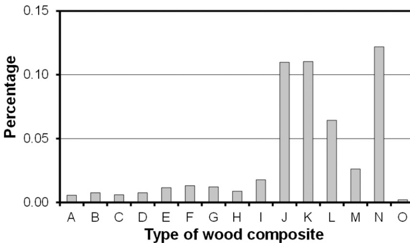
Figure 6. Content percentages of dust particles with a size smaller than 1 μm in the dust created during the milling of wood composites (C 1 μm).
