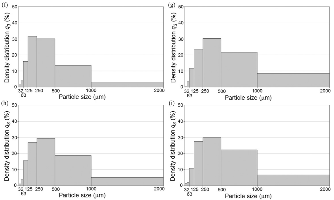
Figure 4. Particle-size distribution of dust from milling of wood composites made of chips obtained by sieve analysis.
