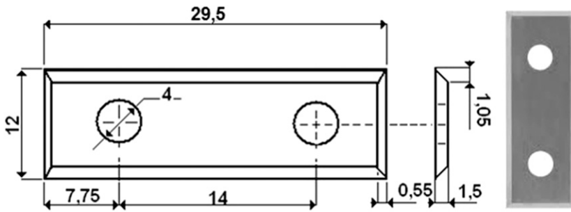
Figure 2. Geometry of the cutting edge.
