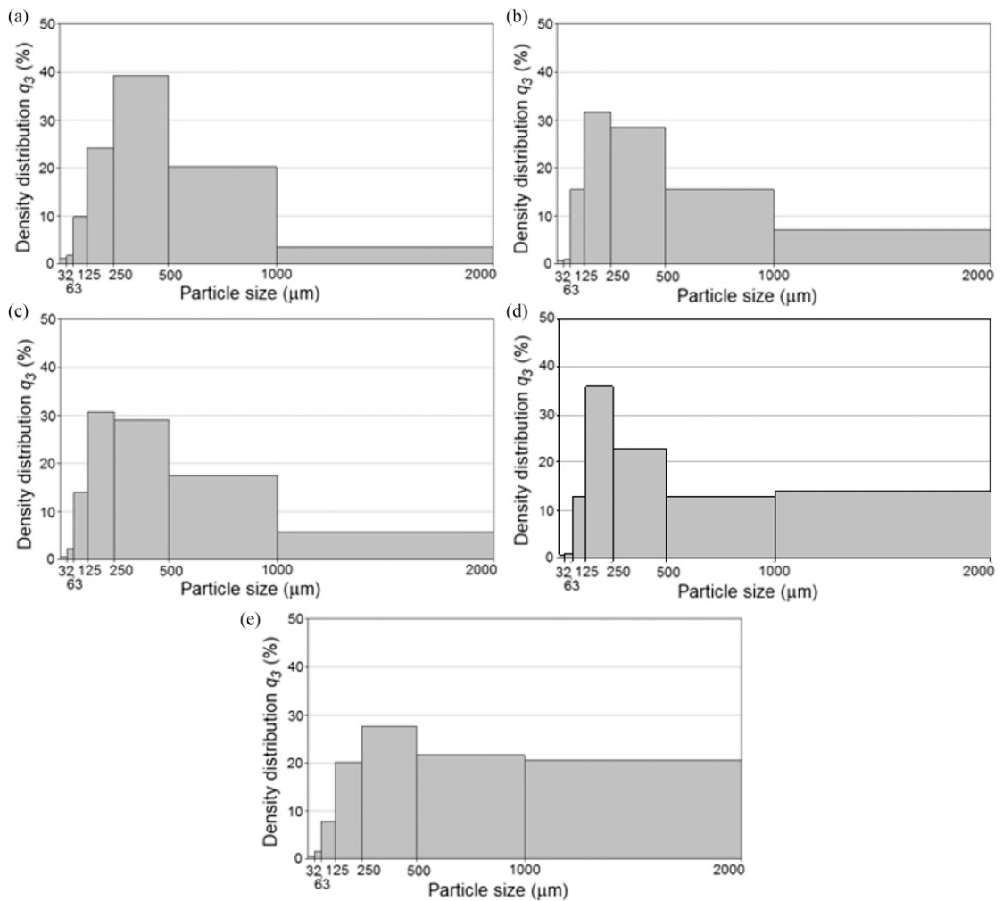
Figure 3. Particle-size distribution of dust from milling of layered boards obtained by sieve analysis.
