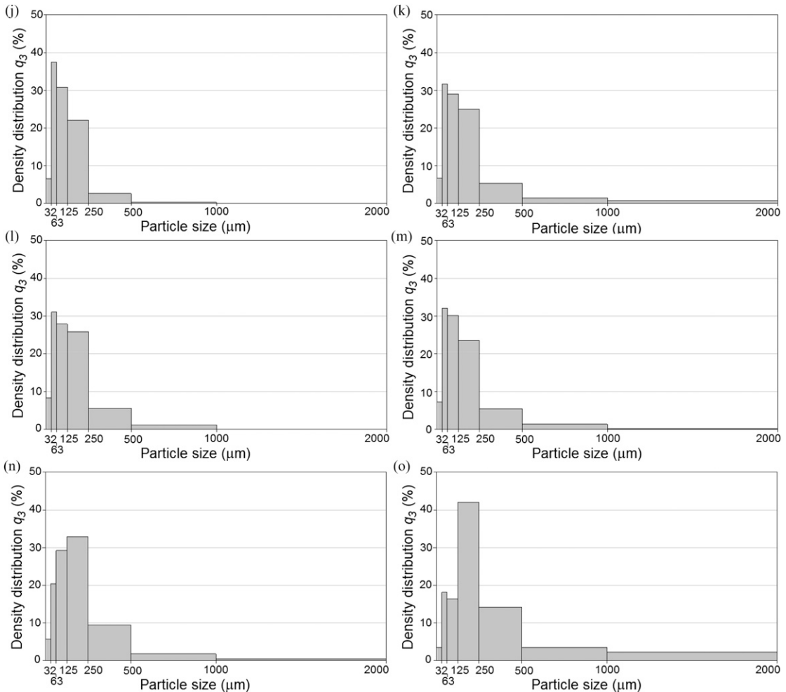
Figure 5. Particle-size distribution of dust from milling of wood composites made of fibers obtained by sieve analysis.
