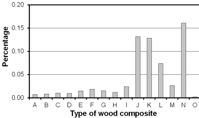
Figure 7. Content percentages of dust particles with a size of 1-2.5 \mu\text{m} in the dust created during the milling of wood composites ( C_i = 1-2,5 \mu\text{m} ).
