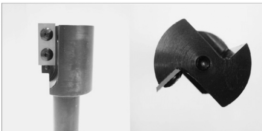
Figure 1. Cutter head.
